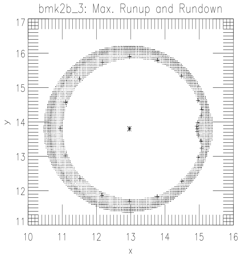
Figure 14. Predicted (dots) shoreline positions for case B of Benchmark Problem 2 of Yeh et al. [1996]. Thus the dotted region shows the region between maximum run-up and run-down during the run. The crosses denote the measured positions of maximum run-up. Note that each dot corresponds to the center of a wet cell at the shoreline.
