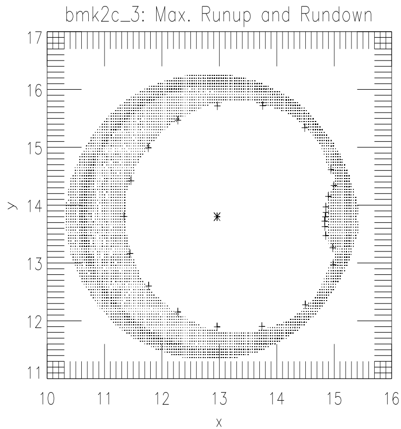
Figure 16. Predicted (dots) shoreline positions for case C of Benchmark Problem 2 of Yeh et al. [1996]. Thus the dotted region shows the region between maximum run-up and run-down during the run. The crosses denote the measured positions of maximum run-up. Note that each dot corresponds to the center of a wet cell at the shoreline.
