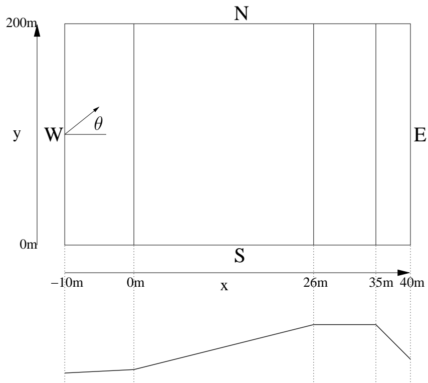
Figure 19. Plan view and cross-section of the numerical wave basin for the (1:4) Q1425 2D overtopping tests.
