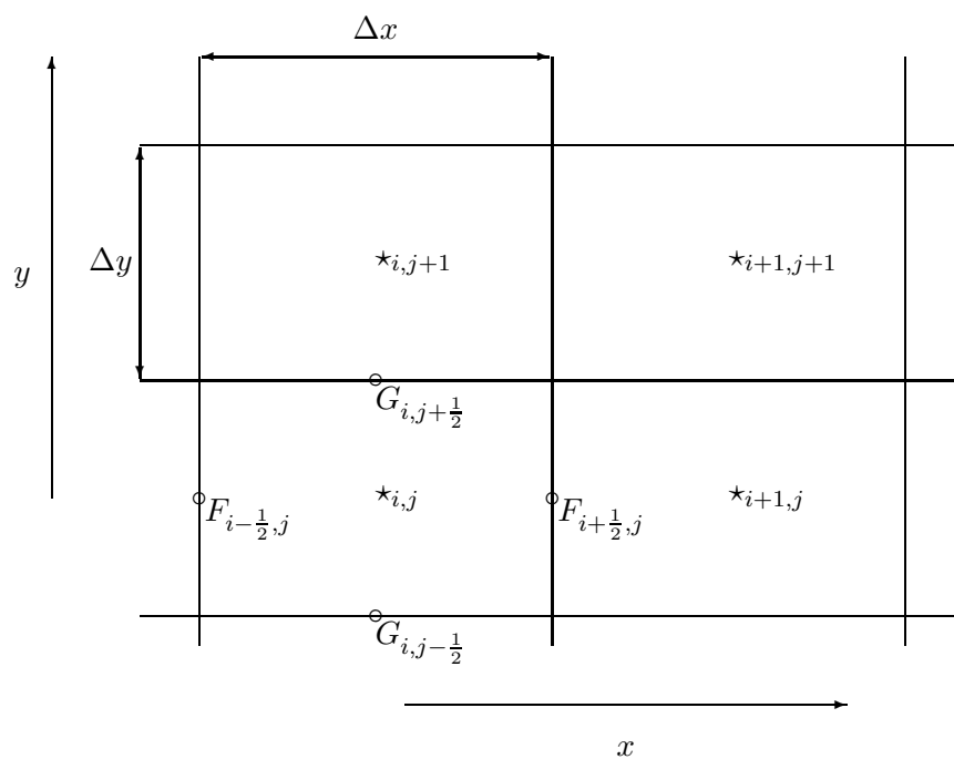
Figure 2. The structured solution grid. \star indicates a cell center, at which location conserved variables are stored; \circ denotes a cell edge (interface) center, at which fluxes are evaluated.
