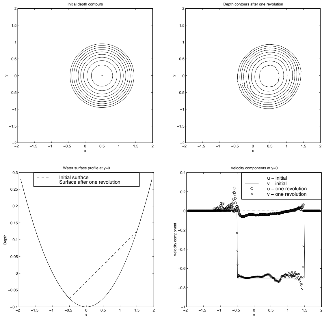
Figure 7. Comparison of the numerical approximation to the flow around a parabolic basin with the exact NLSW solution after a single revolution (the same as the initial conditions). The top two diagrams show contours of water depth for both exact and approximate solutions. The bottom two give comparisons of free surface elevation, overlaid on the bed geometry, (left) and velocity components (right) along the line y = 0 .
