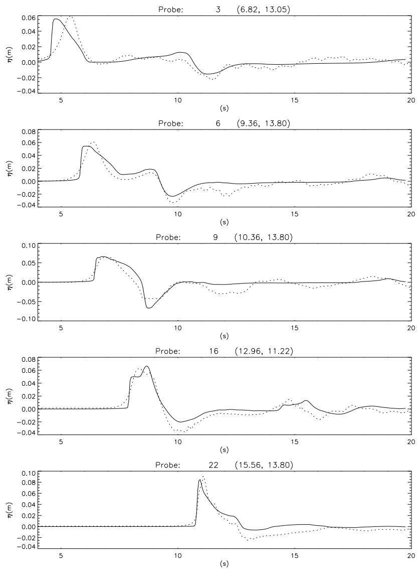
Figure 15. Predicted (solid line) and measured (broken line) free surface elevation at wave gages 6, 9, 16 and 22 of Benchmark Problem 2C of Yeh et al. [1996].
