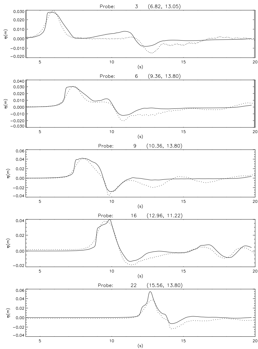
Figure 13. Predicted (solid line) and measured (broken line) free surface elevation at wave gages 6, 9, 16 and 22 of Benchmark Problem 2B of Yeh et al. [1996].
