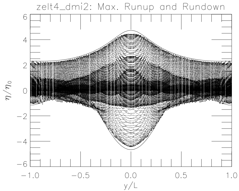
Figure 10. Run-up in 2D: maximum and minimum run-up. Dots indicate the surface elevation ( d(x, y, t) - h(x, y) ) at the center of each shoreline node. The solid line is the maximum run-up and run-down found by Özkan-Haller and Kirby [1997].
