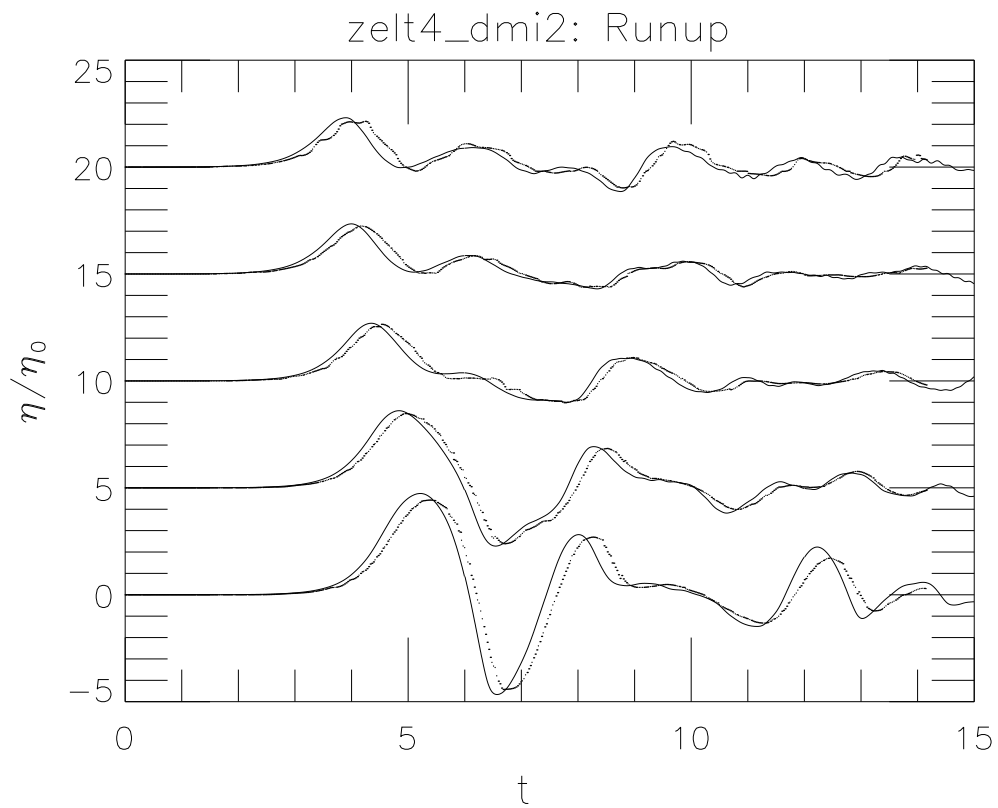
Figure 9. Time series of run-up at 5 alongshore ( y ) locations. Solid line indicates the solution of Özkan-Haller and Kirby [1997]; the dotted line is the present method.
