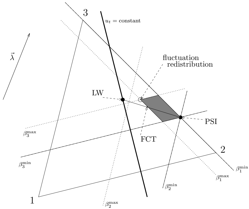
Figure 3.2: A monotonicity region (shaded dark grey) for the distribution point based on the PSI and Lax-Wendroff schemes.
