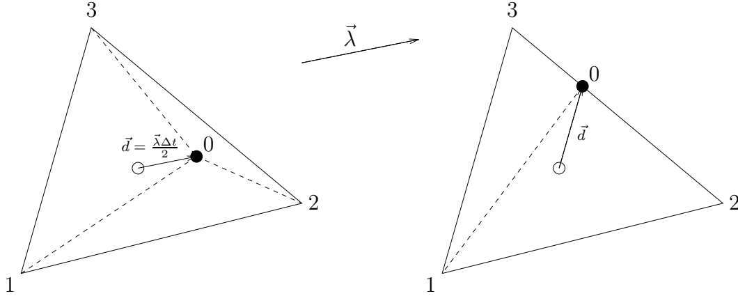
Figure 3.1: The position of the distribution point for the Lax-Wendroff scheme (left) and in the two-target case for a fully upwind scheme, e.g. PSI (right).
