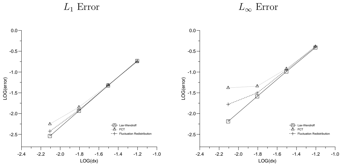
Figure 4.6: Errors for the double sine wave test case on grid B.
