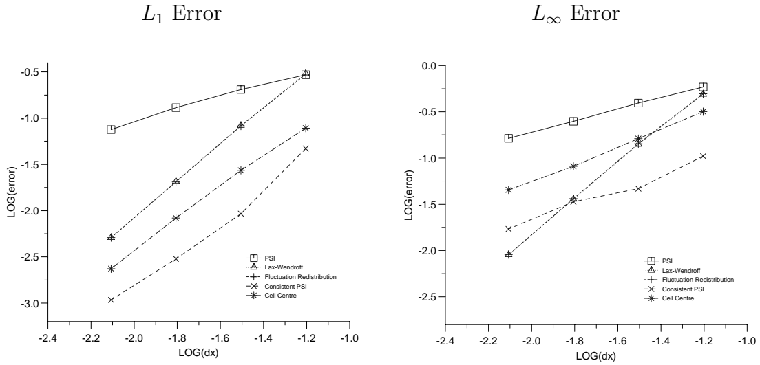
Figure 4.4: Errors for the double sine wave test case on grid A.
