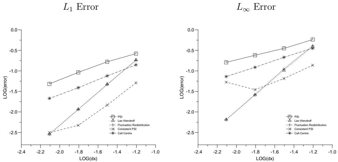
Figure 4.5: Errors for the double sine wave test case on grid B.
