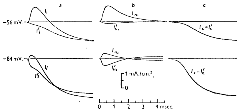
Fig. 5. Curves illustrating separation of ionic current into I_{Na} and I_K . Upper part of figure. a , ionic currents: I_i , axon in sea water, membrane potential lowered by 56 mV.; I'_i , axon in 10% sodium sea water, membrane potential lowered by 60 mV. (average of curves taken before and after I_i ). b , sodium currents: I_{Na} , sodium current in sea water; I'_{Na} , sodium current in 10% sodium sea water. c , potassium current, same in both solutions. Lower part of figure. Same, but membrane potential lowered by 84 mV. in sea water and 88 mV. in 10% sodium sea water. Current and time scales same for all curves. Axon no. 21; temperature 8.5° C.
