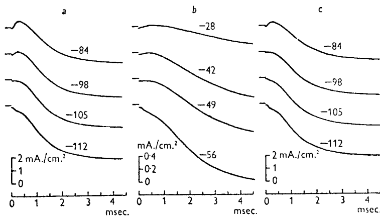
Fig. 4. Curves of ionic current density during voltage clamps in neighbourhood of sodium potential. a , axon in sea water; b , axon in 10% sodium sea water; c , after replacing sea water. Note that ordinate scale is larger in b than in a and c . Displacement of membrane potential in millivolts indicated for each curve. Axon no. 21; temperature 8.5° C.
