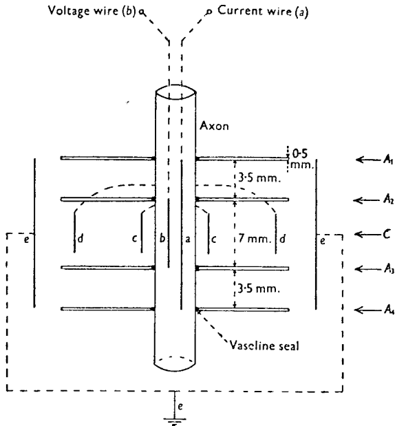
Fig. 1. Diagram illustrating arrangement of internal and external electrodes. A_1 , A_2 , A_3 and A_4 are Perspex partitions. a , b , c , d and e are electrodes. Insulated wires are shown by dotted lines. For sections through A and C , see Figs. 2 and 3.
