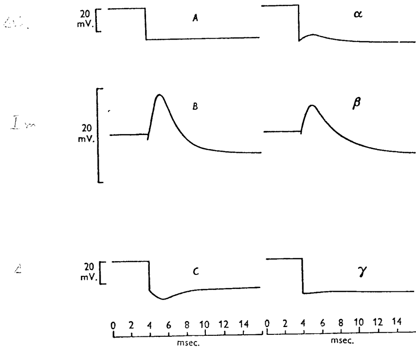
Fig. 17. Comparison of results obtained with uncompensated feed-back ( A, B, C ) and compensated feed-back ( \alpha, \beta, \gamma ). A, \alpha : potential difference between external and internal electrodes ( v_e - v_b ). B, \beta : potential difference between current measuring electrodes ( v_d - v_c ). C, \gamma : membrane potential calculated as C = A - 0.68B , or \gamma = \alpha - 0.68\beta . Records B and \beta may be converted into membrane current density by dividing by 11.9 \Omega \cdot \text{cm}^2 . Temperature 4^\circ \text{C} . Axon 34.
