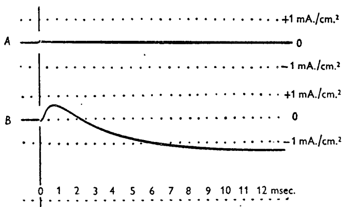
Fig. 11. Records of membrane current under a voltage clamp. At zero time the membrane potential was increased by 65 mV. (record A) or decreased by 65 mV. (record B); this level was then maintained constant throughout the record. Inward current is shown as an upward deflexion. Axon 41; diameter 585 \mu . Temperature 3.8° C. Compensated feed-back.
