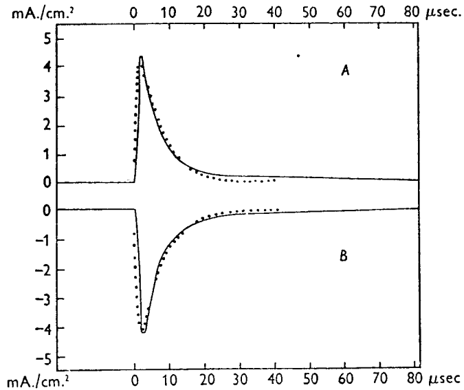
Fig. 16. Current through capacitive element of membrane during a voltage clamp. Abcissa: time in \mu sec. Ordinate: membrane current density ( \text{mA./cm.}^2 ) with inward current taken as positive. At t=0 the potential difference between external and internal electrodes was displaced +40 mV. in curve A or -40 mV. in curve B. The continuous curves were traced from experimental records. The dotted curves were calculated according to the equation
