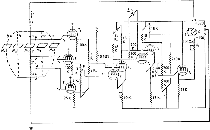
Fig. 6. Schematic diagram of feed-back amplifier. Screen resistances, grid stoppers and other minor circuit elements have been omitted. T_1, T_2, T_3 and T_8 are cathode followers; T_4, T_5, T_6 and T_7 are d.c. amplifiers. All valves were 6AK5 except T_1 and T_2 which were 1223. G is a microammeter used in setting-up. S is a switch for short-circuiting G . M_c is the membrane in the central section of the guard system. M_g , membrane in guard channels. M_o , membrane outside guard system. i_c, i_p and i_o are currents through these elements. r_{cd} , fluid-resistance used to measure current ( 74 \Omega . at 20^\circ \text{C} .). r_s , resistance in series with membrane (about 52 \Omega . at 20^\circ \text{C} .). z_{de} , impedance of large earthed electrode and sea water between d and e . Potentials are given with respect to earth.
