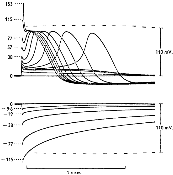
Fig. 8. Time course of membrane potential following a short shock at 23° C. Depolarizations shown upwards. Axon 18. The numbers attached to the curves give the strength of shock in m\mu\text{coulomb/cm}^2 . Shock strengths for unlabelled curves are 29, 23, 19.2, 17.3, 16.7, 15.3, 9.6.
