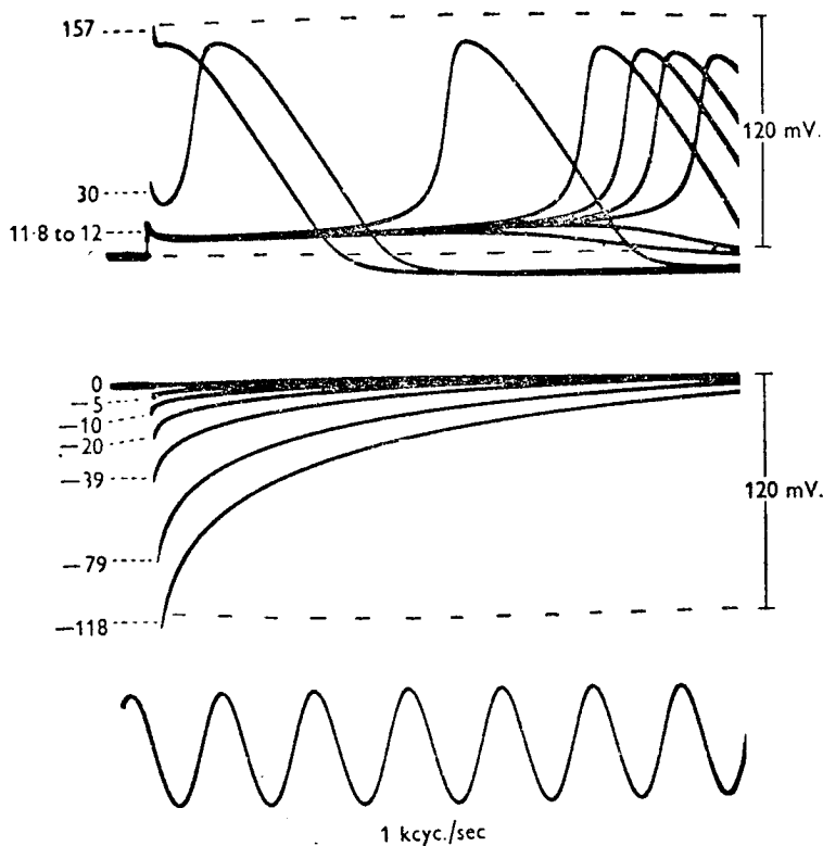
Fig. 9. Time course of membrane potential following a short shock at 6^\circ\text{C} . Depolarization shown upwards. Axon 17. The numbers attached to the curves give the strength of shock in m\mu\text{coulomb/cm.}^2 . The initial displacement in the case of the uppermost curve cannot be seen; its value was about 200 mV.
