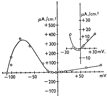
Fig. 10. Relation between ionic current density ( I_i ) and displacement of membrane potential ( V ). Abscissa: displacement of membrane potential from its resting value (anodal displacement shown positive). Ordinate: ionic current density obtained from -C_M \frac{dV}{dt} (inward current shown positive). Inset: curve in region of origin drawn with tenfold increase in vertical scale. Axon 17; C_M=0.74 \mu\text{F./cm.}^2 ; temperature 6.3^\circ \text{C} . Measurements made 0.29 msec. after application of shock.
